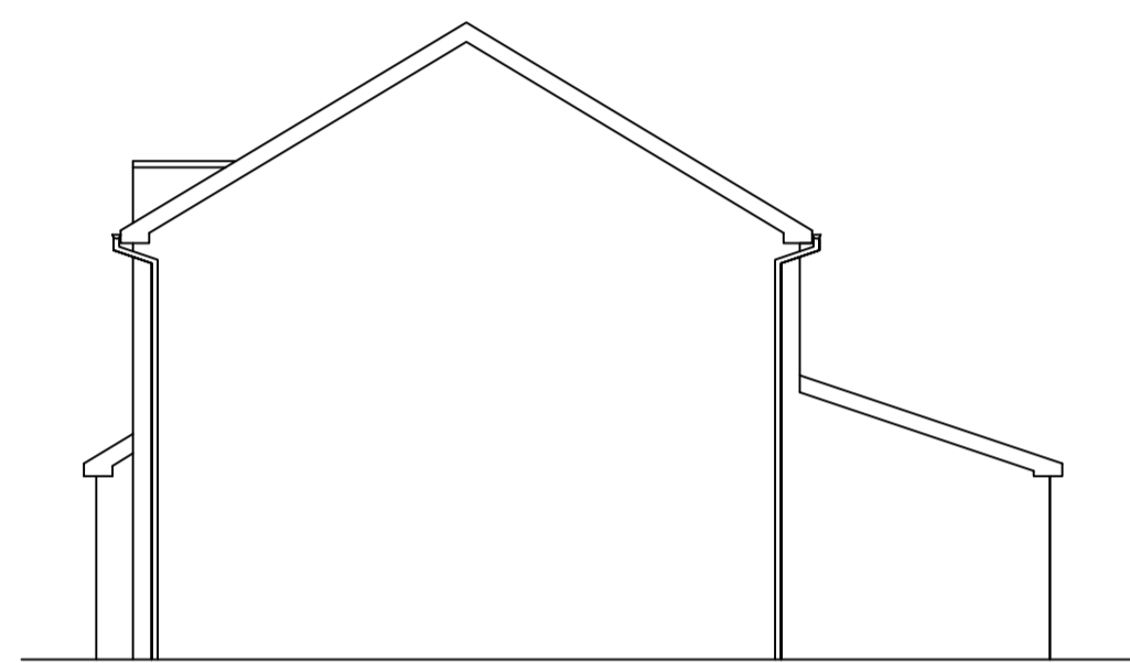
PROPOSED SIDE ELEVATION ON 'C'
