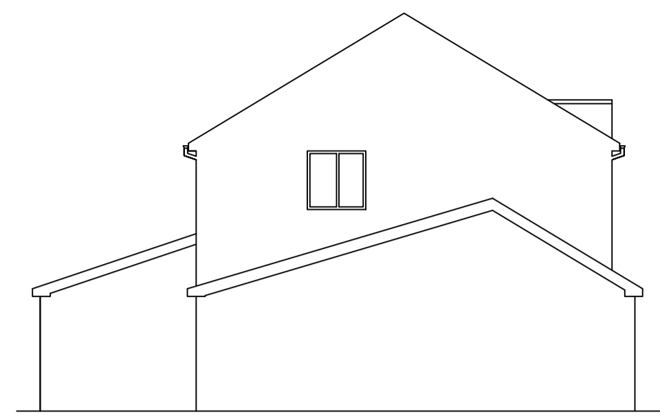
EXISTING SIDE ELEVATION ON 'B'
